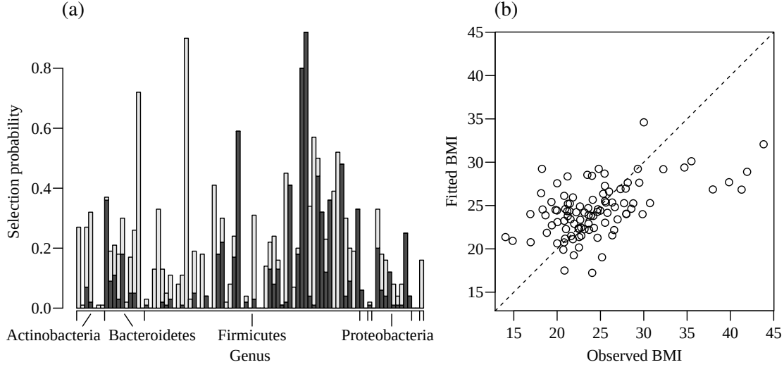
Fig. 1. Analysis of gut microbiome data. (a) Selection probabilities with bootstrapped crossvalidation for 87 genera that belong to eight phyla. Selections with a positive sign and a negative sign are shown by dark grey blocks and light grey blocks, respectively; only four major phyla are indicated. (b) Fitted versus observed values of BMI.
