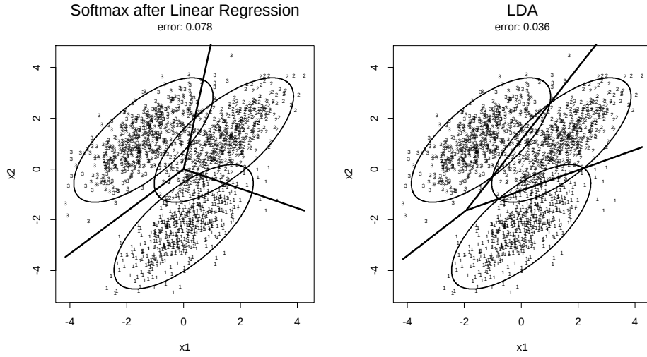
Figure 5: Softmax uses the wrong metric. The data consist of 500 samples each from 3 bivariate Gaussian distributions, differing in location, but with the same covariance structure. The location of their centroids distorts S_T relative to S_W , and results in a biased decision boundary for softmax on the left, while not for LDA on the right.
