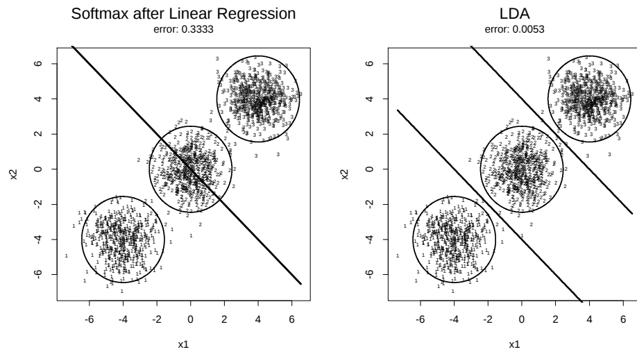
Figure 6: Softmax uses the wrong threshold. The data consist of 500 samples each from 3 spherical bivariate Gaussian distributions, whose centroids line up along a line. The center class is completely masked by the outside two when softmax is used, while LDA has no such problem.
