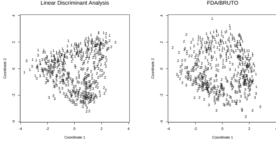
Figure 3: The left plot shows the canonical variates derived from LDA for the waveform data, evaluated for the test data; the classes are numerically coded. The right plot is the same, but derived from the FDA/BRUTO model.
