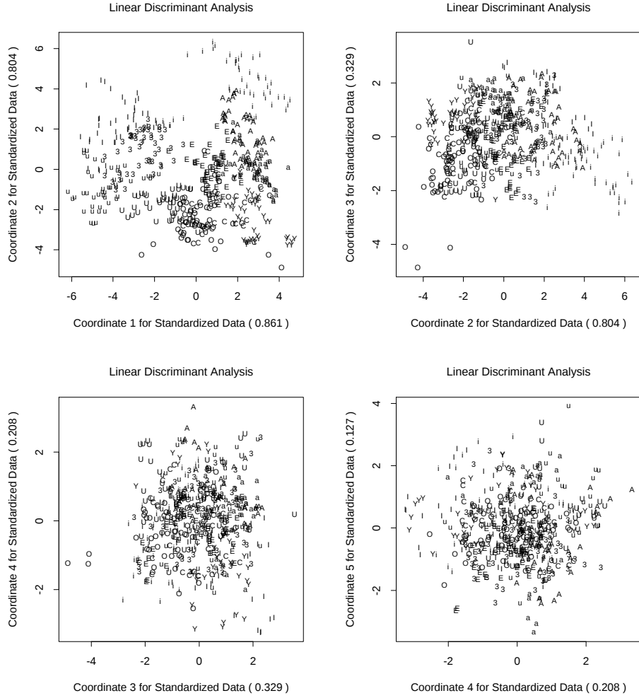
Figure 1: Some selected 2-dimensional projections of the LDA subspace computed for the vowel data described in section 3.4; the eigenvalues for each coordinate are in parentheses, and indicate the strength of that variable in separating the groups. These plots show visually that most of the discrimination lies in the first few discriminant variables.
