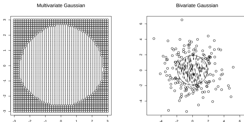
Figure 2: The left plot shows a view of the decision boundary for the ten-dimensional Gaussian example fit using the BRUTO procedure, obtained by setting coordinates 3-10 to zero. The plot symbols are “I” or “O” for inner and outer, produced over a uniform grid in this two-dimensional slice. The right plot shows the predicted class and the Bayes-optimal decision boundary for the two-dimensional Gaussian example.
