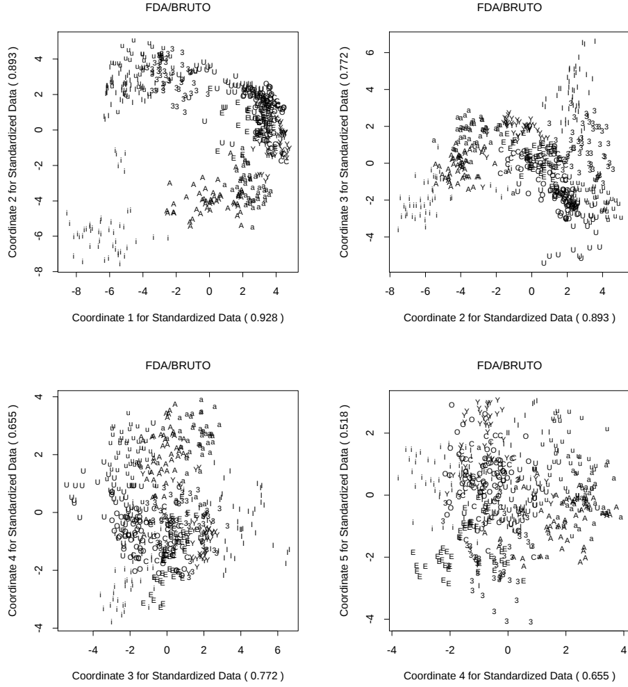
Figure 4: Some selected 2-dimensional projections of the canonical variates derived from the FDA/BRUTO model fit to the vowel data; the eigenvalues for each coordinate are in parentheses, and indicate the strength of that variable.
